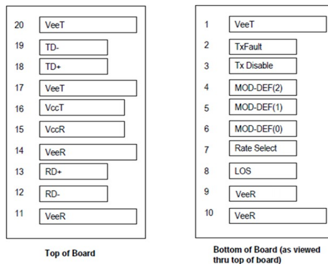
Pin-out of connector Block on Host board
